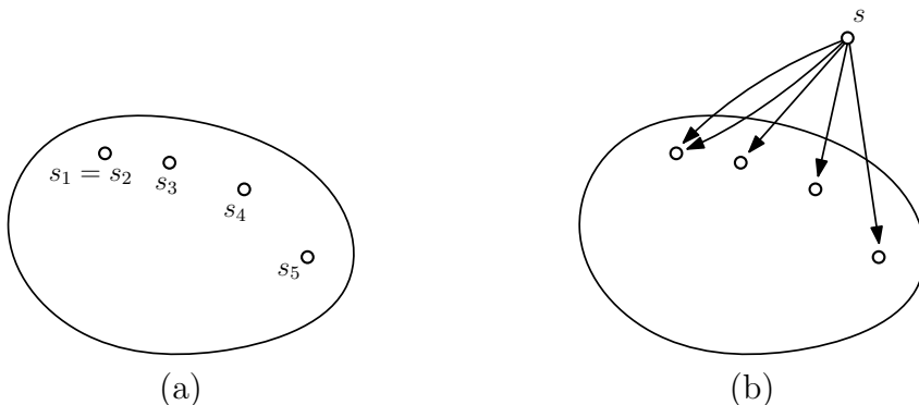
Figure 2: (a) A digraph D' with a multiset of roots and (b) the corresponding rooted digraph D .
