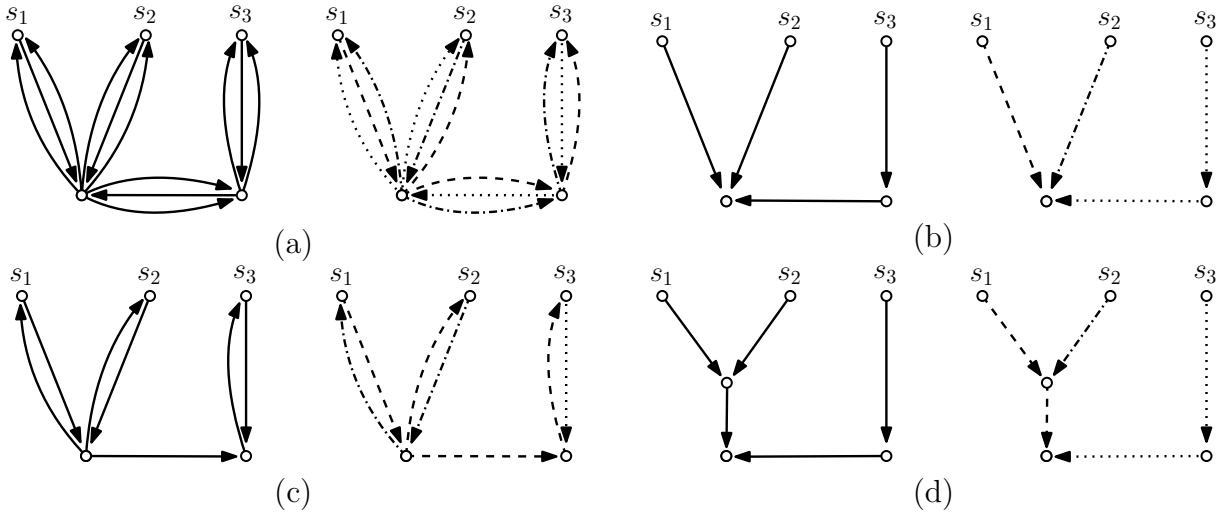
Figure 1: Examples of arborescence packings, where the left figure is a given digraph with the root set \{s_1, s_2, s_3\} and the right figure indicates a packing. The uniform matroid \mathcal{M} of rank two is given on \{s_1, s_2, s_3\} . (a) a packing of spanning arborescences, (b) a reachability packing of arborescences, (c) an \mathcal{M} -based packing of arborescences, and (d) an \mathcal{M} -reachability-based packing of arborescences.
