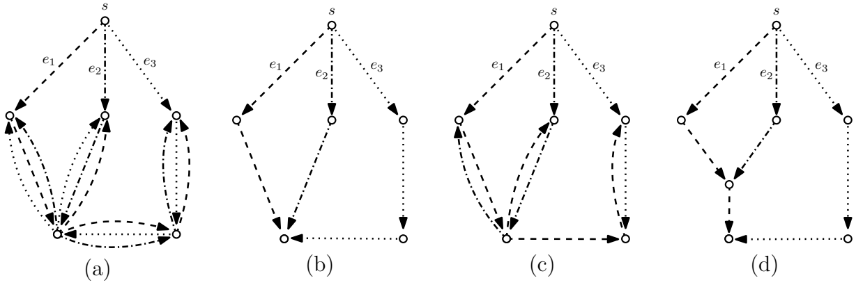
Figure 3: Packings of s -arborescences in rooted digraphs corresponding to the examples in Figure 1. The uniform matroid \mathcal{M} of rank two is given on the set \{e_1, e_2, e_3\} of root arcs.
