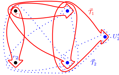
Fig. 2. \vec{T}_1 is a spanning r_1 -hyperarborescence while \vec{T}_2 is a reachability r_2 -hyperarborescence of the dypergraph.
