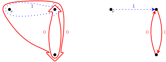
Fig. 4. The trimming operation does not preserve minimum cost arborescence packings.
