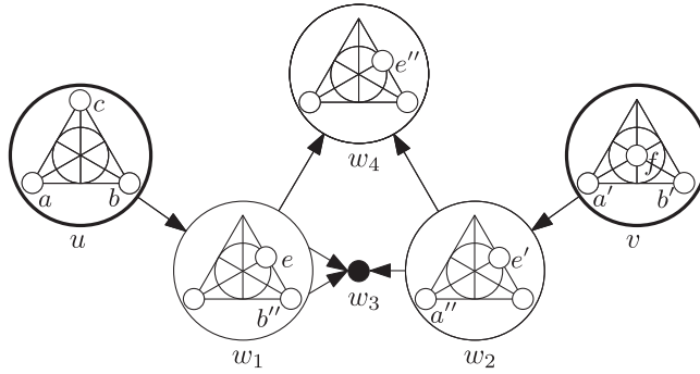
FIGURE 7 An example of FSC_{(a,b')}(u, v) , where (x, y, z) = (b', a', f) and t = e .
