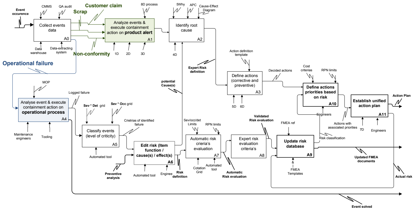
Figure 6 Proposed process for unified action plan
