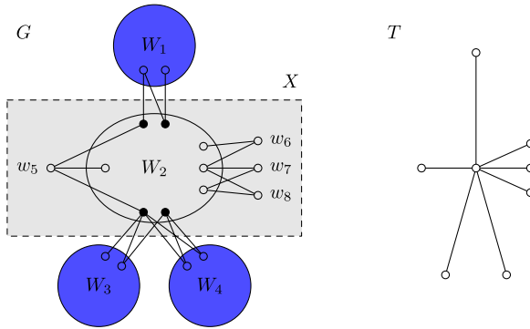
Fig. 1 Schematic illustration of a graph G (on the left) that is contractible to tree T (on the right). The sets W_1, W_2, W_3 and W_4 are connected, and G itself is 2-connected; for simplicity, not all vertices and edges have been drawn. Let \mathcal{W} be the T -witness structure of G with four big witness sets W_1, \dots, W_4 and four small witness sets \{w_5\}, \dots, \{w_8\} . Let \phi be a \mathcal{W} -compatible 2-coloring of G that colors the dark shaded (blue in the online version) big witness sets W_1, W_2, W_3, W_4 with one color, and the other sets of \mathcal{W} with the other color. The set \mathcal{X} of monochromatic components of \phi forms a T'' -witness structure of G , where T'' is a star with three leaves. Consider the monochromatic component X of \phi that is indicated in the figure. The four witness sets of \mathcal{W} that are contained in X form a shatter of X , but not necessarily a minimum shatter of X . The four black vertices form the set \hat{X}
