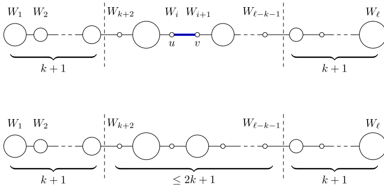
Fig. 4 Illustration for the proof of Lemma 4. If among the witness sets W_{k+2}, \dots, W_{\ell-k-1} two consecutive witness sets W_i and W_{i+1} are small (top), then Rule 1 can be applied on the instance (G, k) . If no two consecutive witness sets among W_{k+2}, \dots, W_{\ell-k-1} are small (bottom), then \ell \leq 4k + 3
