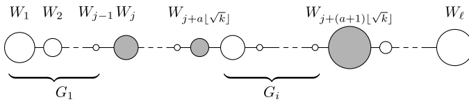
Fig. 5 Schematic illustration of the P_\ell -witness structure \mathcal{W} of G , mentioned in the correctness proof of the algorithm in Theorem 7. The shaded witness sets form the set W_j^* . The vertices in the sets W_1, \dots, W_{j-1} induce the graph G_1 , which is an end-component of G - W_j^* . Let G_i be a connected component of G - W_j^* that is not an end-component, i.e., G_i is the graph induced by the vertices of those witness sets of \mathcal{W} that appear between the sets W_{j+a\lfloor\sqrt{k}\rfloor} and W_{j+(a+1)\lfloor\sqrt{k}\rfloor} for some integer a . Note that these witness sets W_{j+a\lfloor\sqrt{k}\rfloor+1}, \dots, W_{j+(a+1)\lfloor\sqrt{k}\rfloor-1} constitute a P_{\lfloor\sqrt{k}\rfloor-1} -witness structure \mathcal{X}_i of G_i
